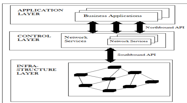
Fig. 1. SDN Architecture
