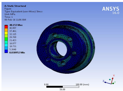
Fig.4 von-Mises stress at the wheel hub
